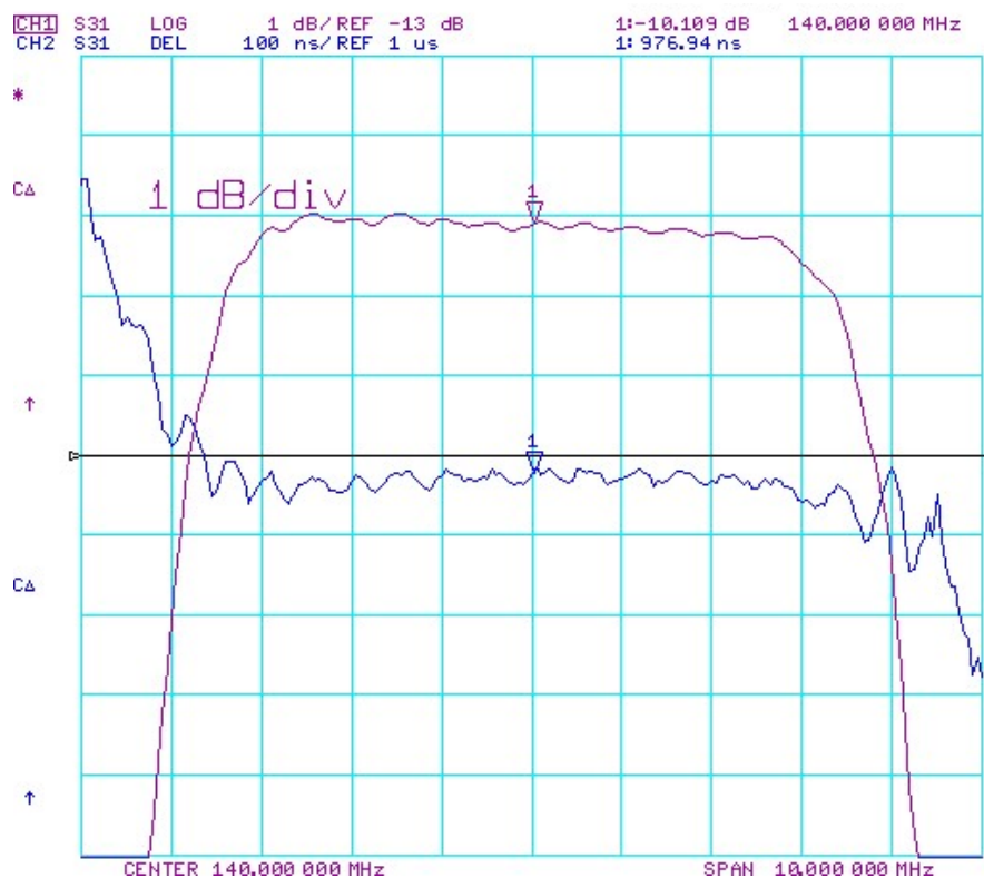
Fig2.S21 Response Horizontal:1MHz/Div Vertical: 1dB/Div
